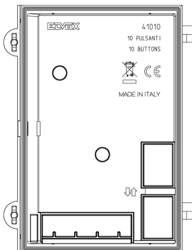
Backside view
